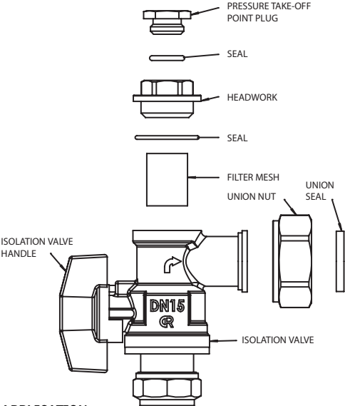
Exploded view of UA angle valve assembly
